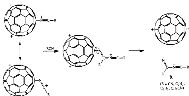
Figure 4. Proposed mechanism for the formation of nitrile dimer cation (RCN)_2^{3+} in the secondary reaction C_{60}(RCN)^{3+} + RCN . As with other reactions of nitriles with fullerene cations, the reaction is thought to involve nucleophilic attack by the nitrile RCN .
